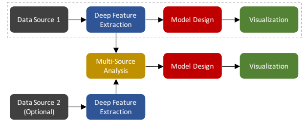
Figure 1. PADDLE – a generic machine learning framework for performance data analysis. The proposed framework is well-suited for a wide-range of problems that require the design of models for predictive or comparative analysis using one or more data sources. In addition to being robust and accurate, the resulting models are also easily interpretable.
