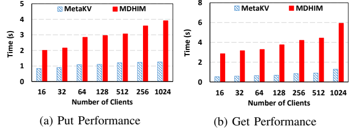
Fig. 10: Index Put and Get Performance with MPI-Tile-IO.
