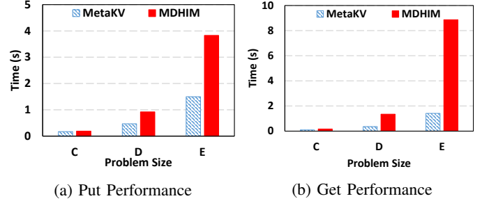
Fig. 11: Index Put and Get Overhead with BTIO.
