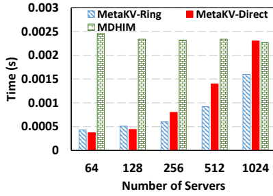
Fig. 12: Performance of Log-Ring Based Collective Messaging
