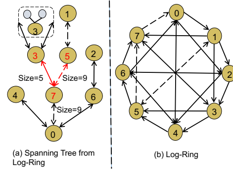
Fig. 7: Log-Ring Based Collective Message Reduction
