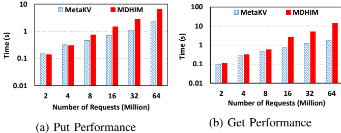
Fig. 9: Index Put and Get Overhead with IOR.
