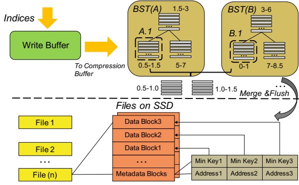
Fig. 4: Compressed Storage Management in MetaKV.
